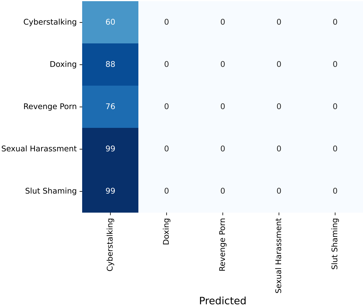
Confusion Matrix
