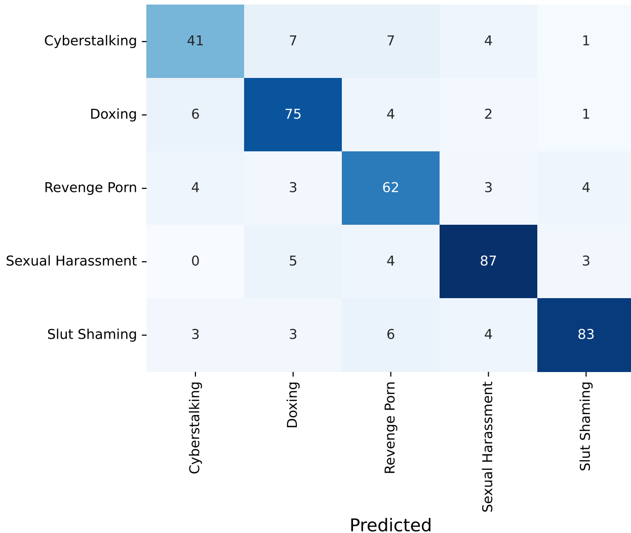
Confusion Matrix
