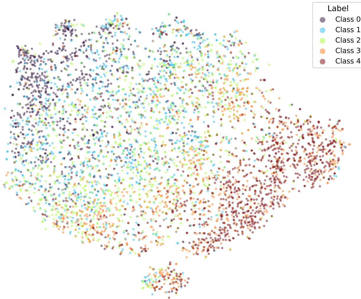
t-SNE | bert-tiny-amazon_reviews-k10-fixed-cosine (epoch 7.0)
