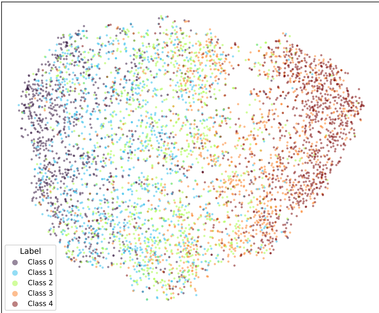
t-SNE | bert-tiny-amazon_reviews-k3-adaptive-cosine (epoch 3.0)
