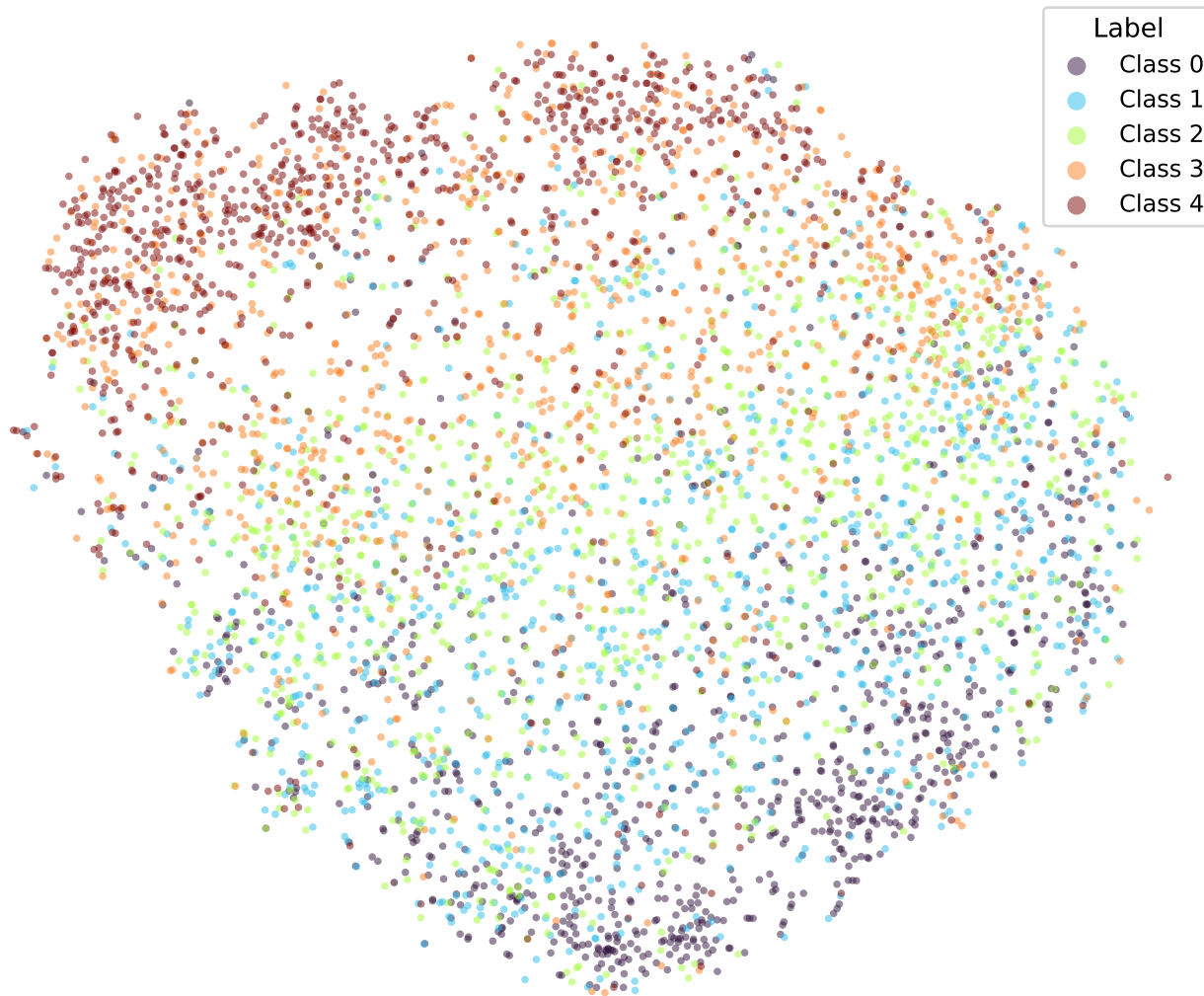
t-SNE | bert-tiny-amazon_reviews-k3-fixed-cosine (epoch 3.0)
