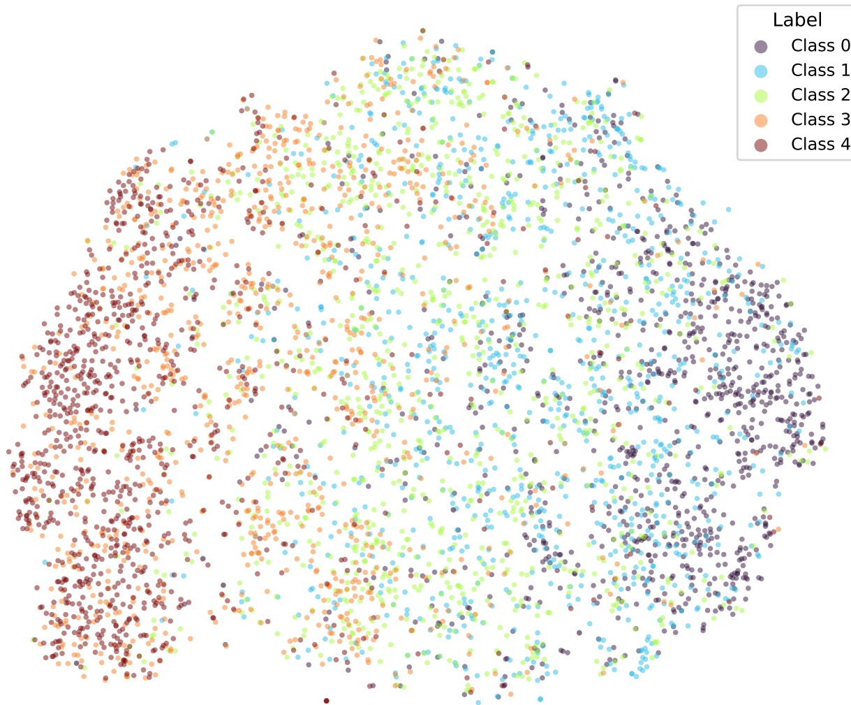
t-SNE | bert-tiny-amazon_reviews-k5-adaptive-cosine (epoch 7.0)
