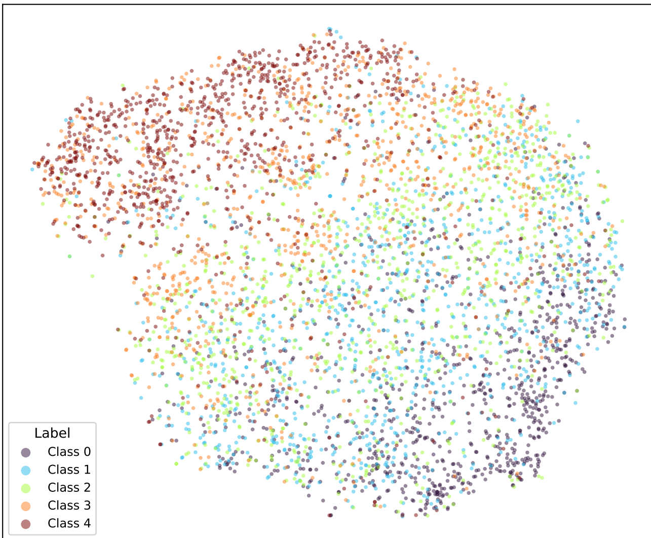
t-SNE | bert-tiny-amazon_reviews-k5-fixed-cosine (epoch 5.0)
