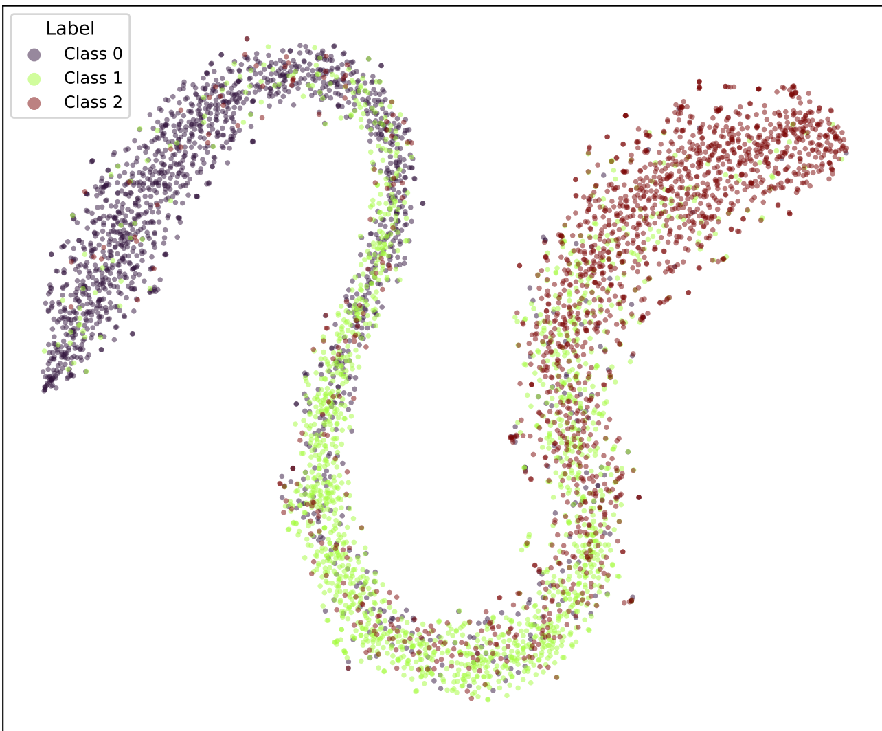
t-SNE | bert-tiny-snli-k1-adaptive-euclidean
