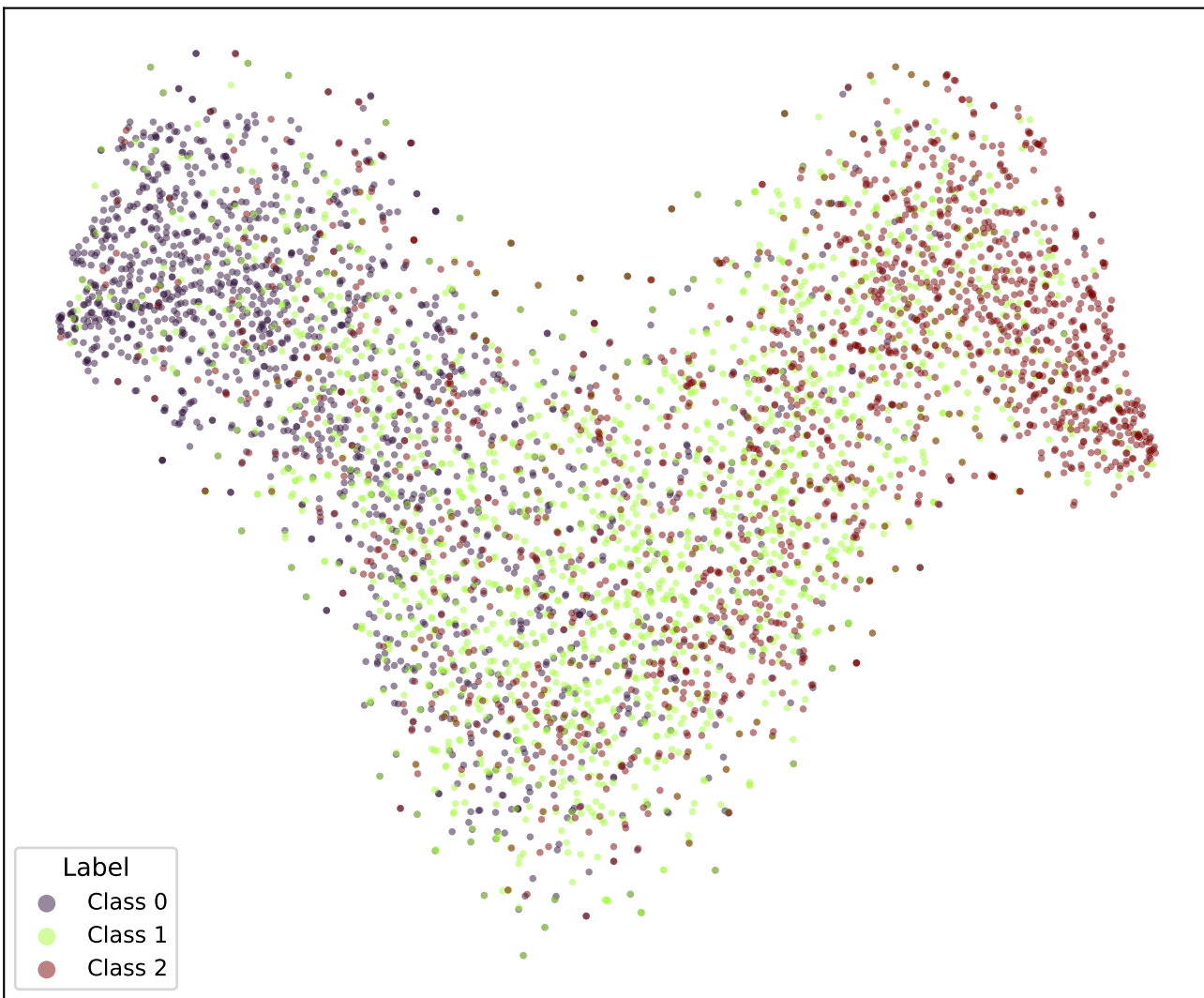
t-SNE | bert-tiny-snli-k1-adaptive-euclidean (epoch 1.0)
