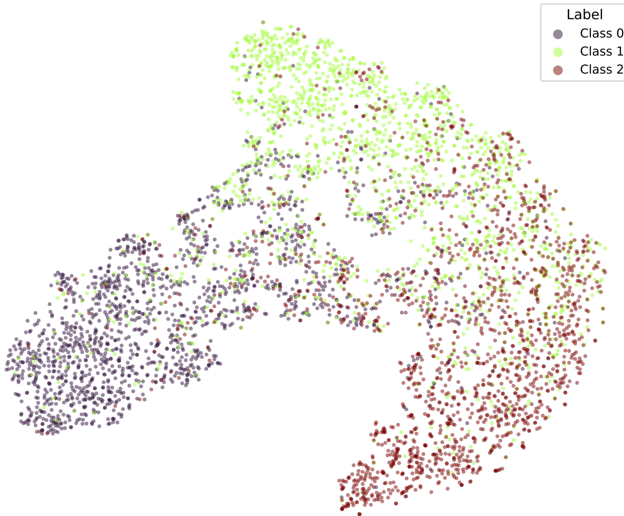
t-SNE | bert-tiny-snli-k1-fixed-euclidean (epoch 5.0)
