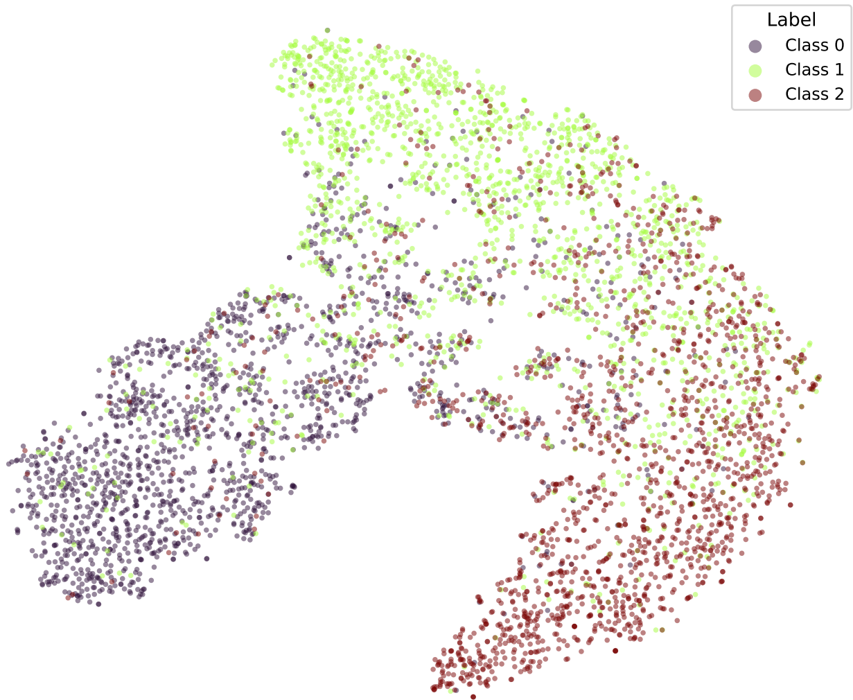
t-SNE | bert-tiny-snli-k1-fixed-euclidean (epoch 7.0)
