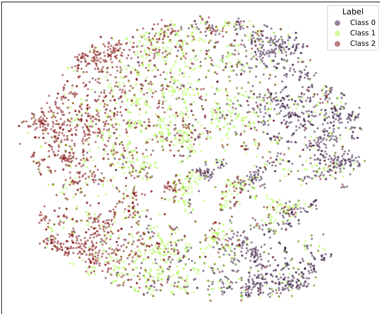
t-SNE | bert-tiny-snli-k10-adaptive-cosine (epoch 1.0)
