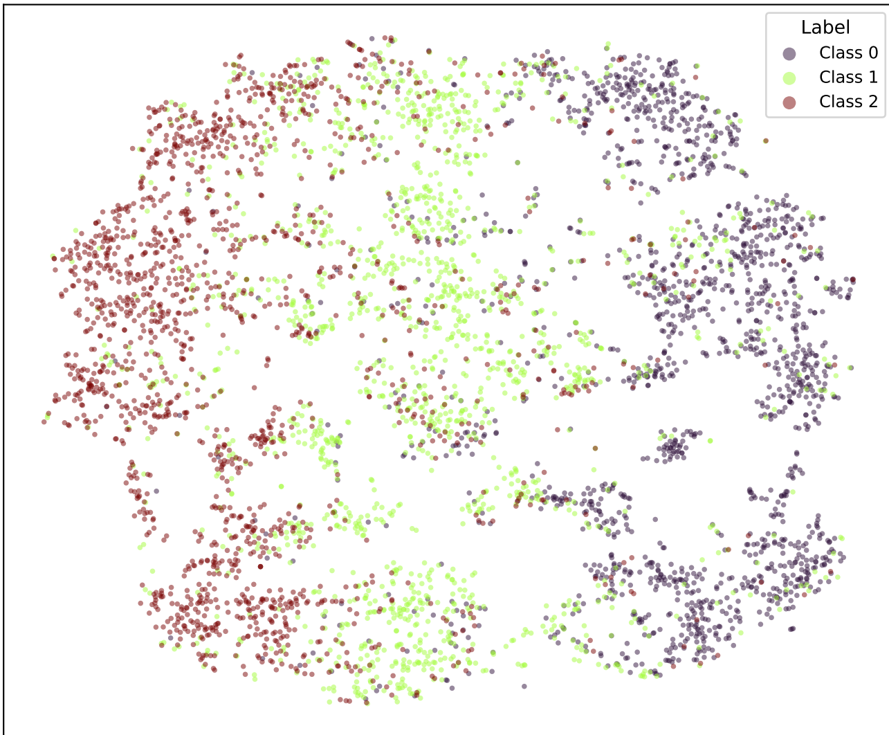
t-SNE | bert-tiny-snli-k10-adaptive-cosine (epoch 5.0)
