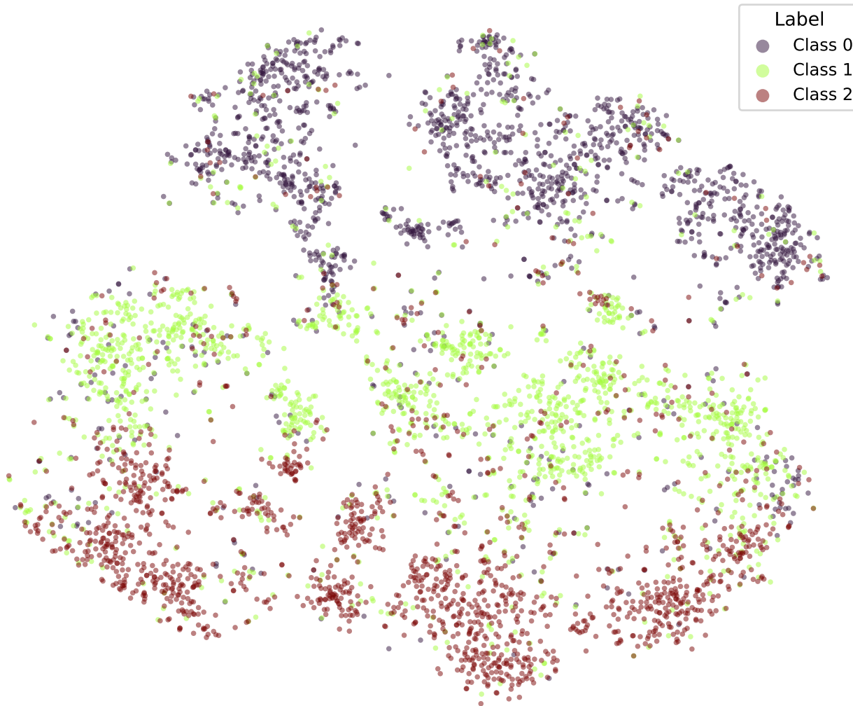
t-SNE | bert-tiny-snli-k10-fixed-cosine (epoch 7.0)
