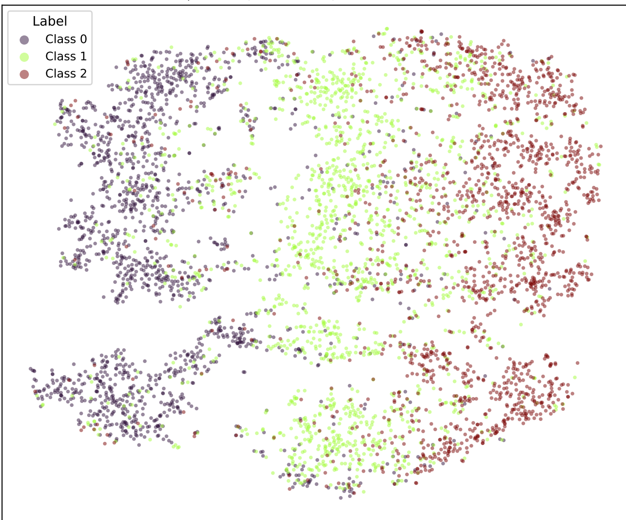
t-SNE | bert-tiny-snli-k5-adaptive-cosine (epoch 5.0)
