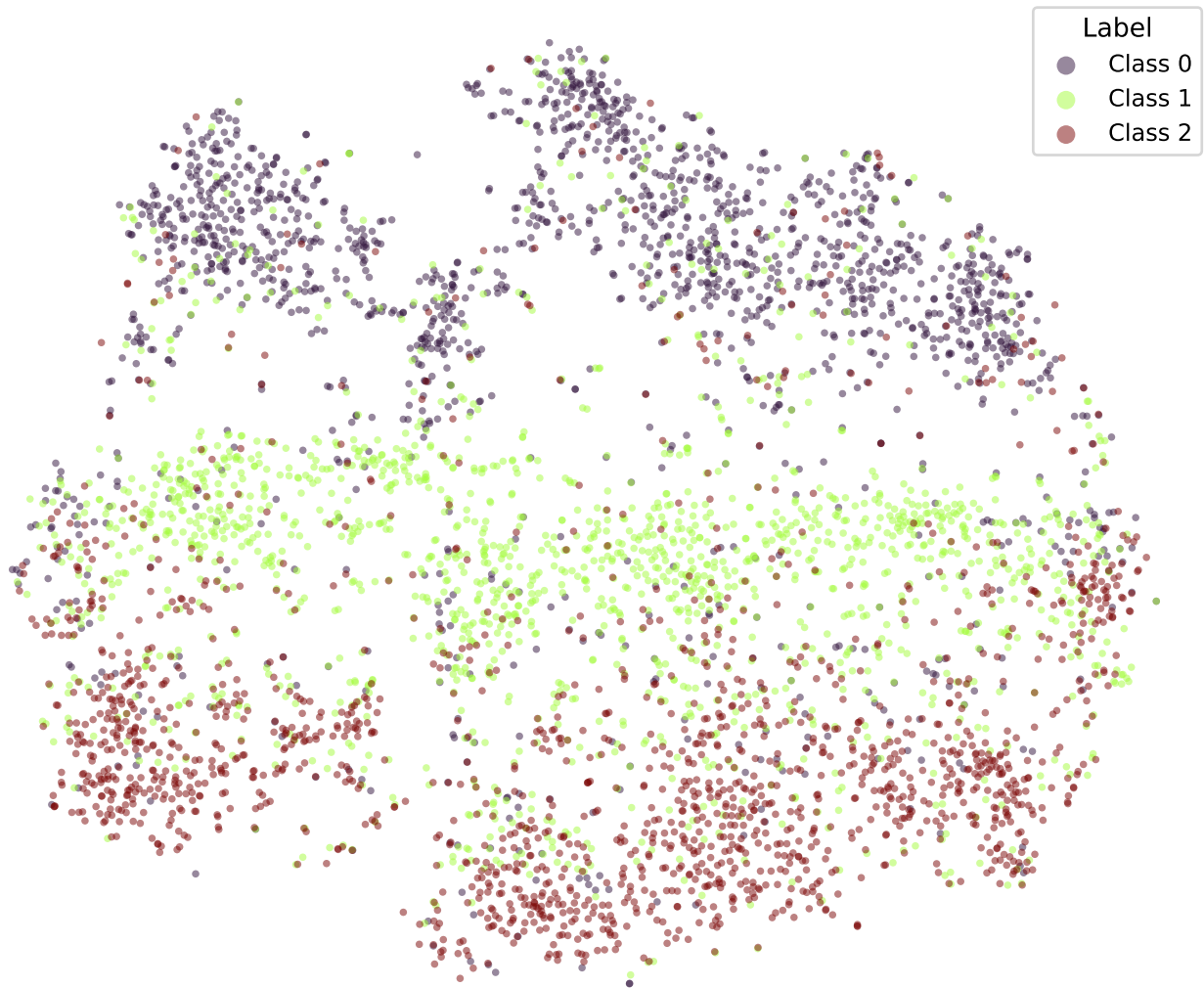
t-SNE | bert-tiny-snli-k5-fixed-cosine (epoch 3.0)
