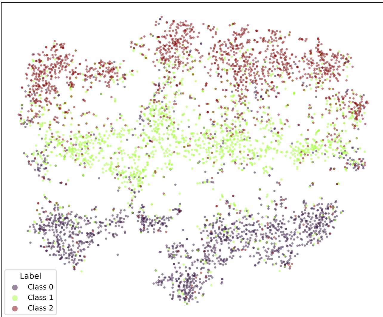
t-SNE | bert-tiny-snli-k5-fixed-cosine (epoch 7.0)
