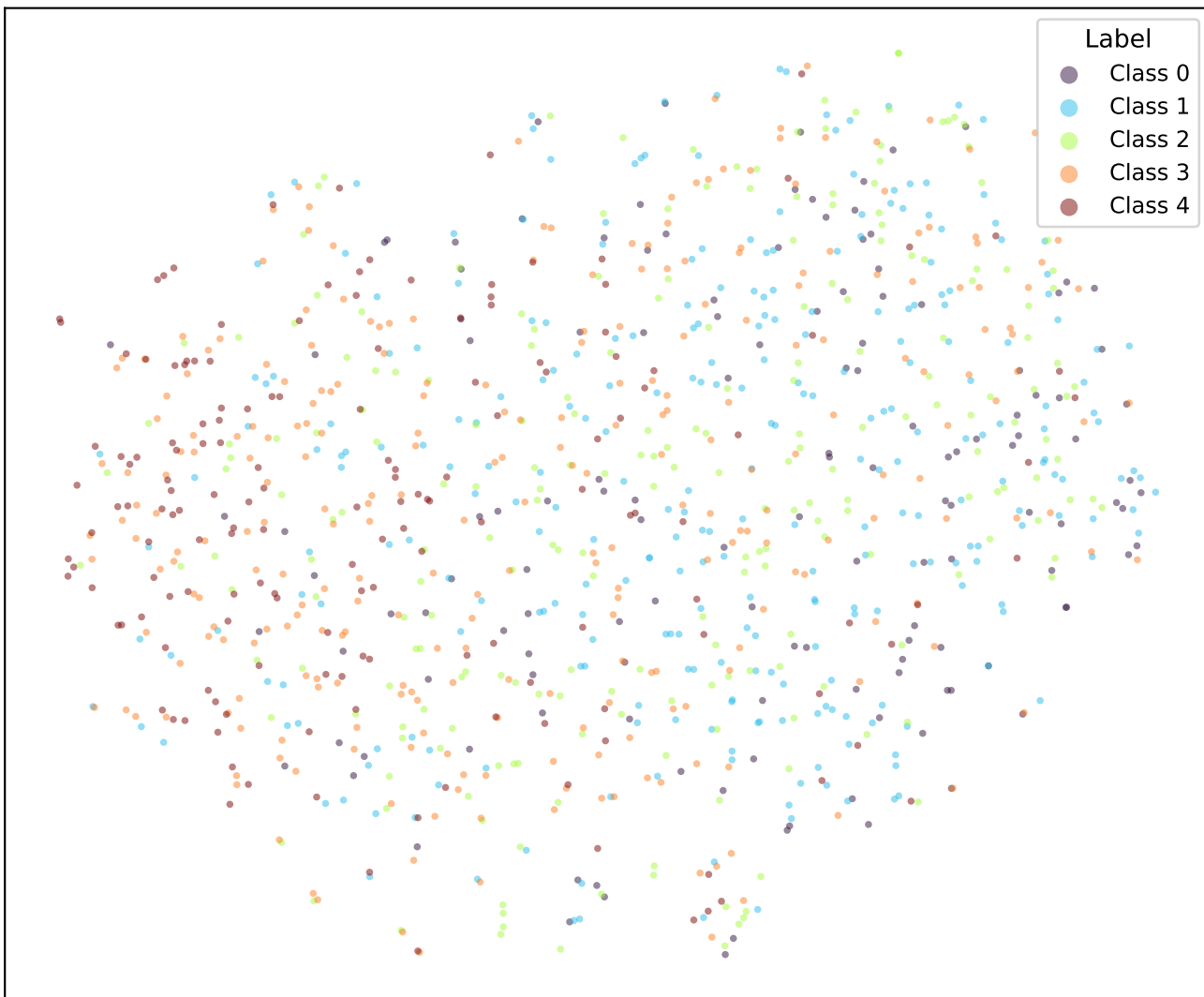
t-SNE | bert-tiny-sst5-k1-adaptive-cosine (epoch 5.0)
