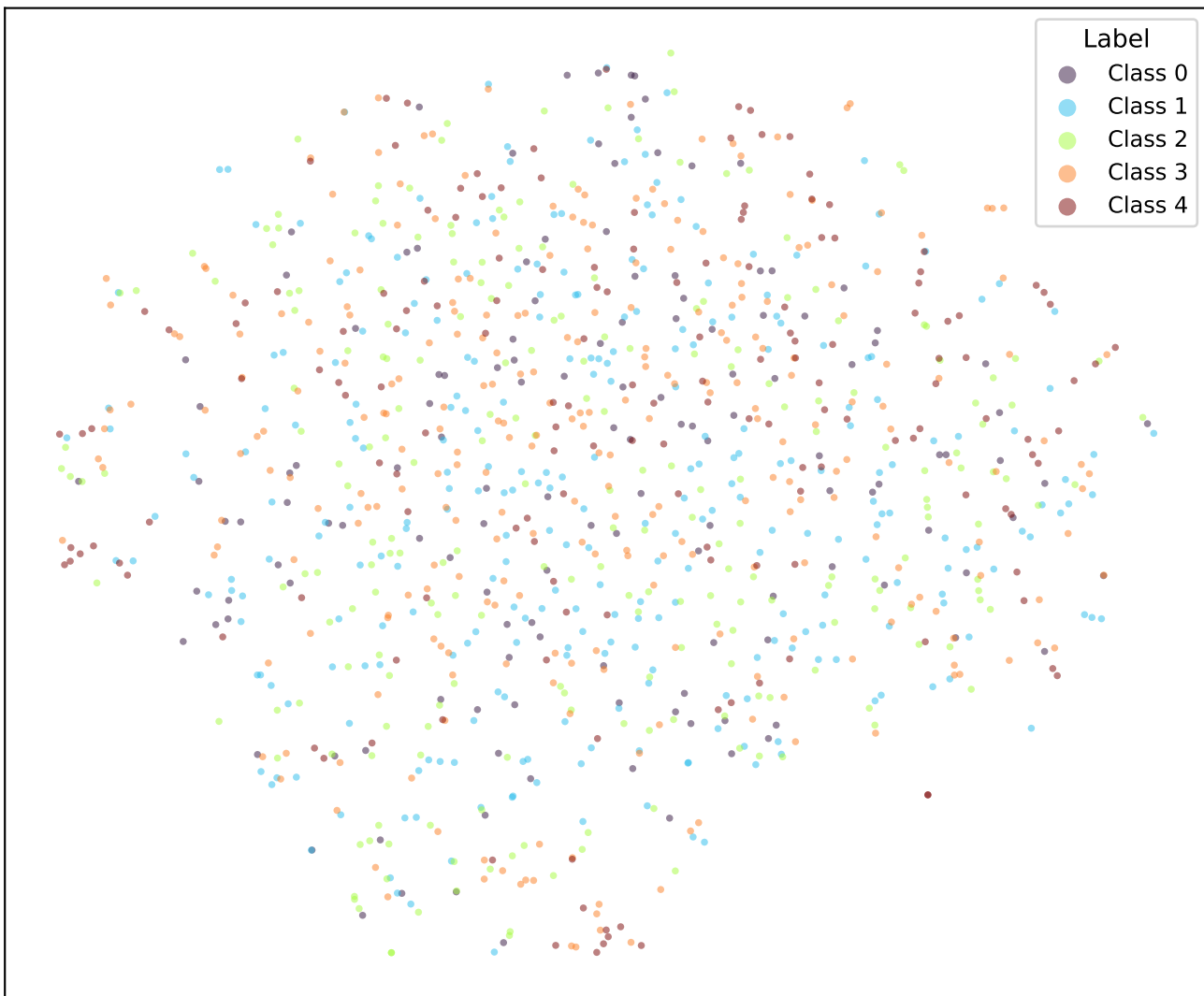
t-SNE | bert-tiny-sst5-k1-adaptive-euclidean (epoch 1.0)
