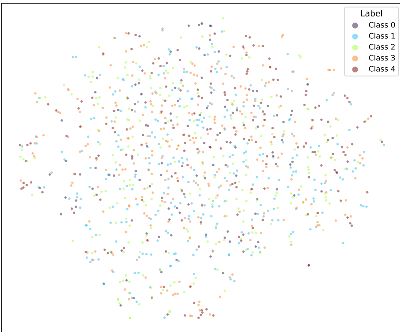
t-SNE | bert-tiny-sst5-k1-fixed-euclidean (epoch 1.0)
