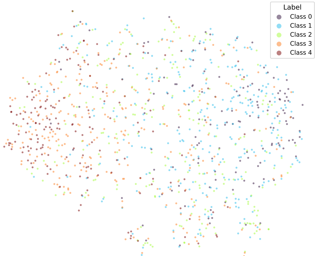
t-SNE | bert-tiny-sst5-k10-adaptive-cosine
