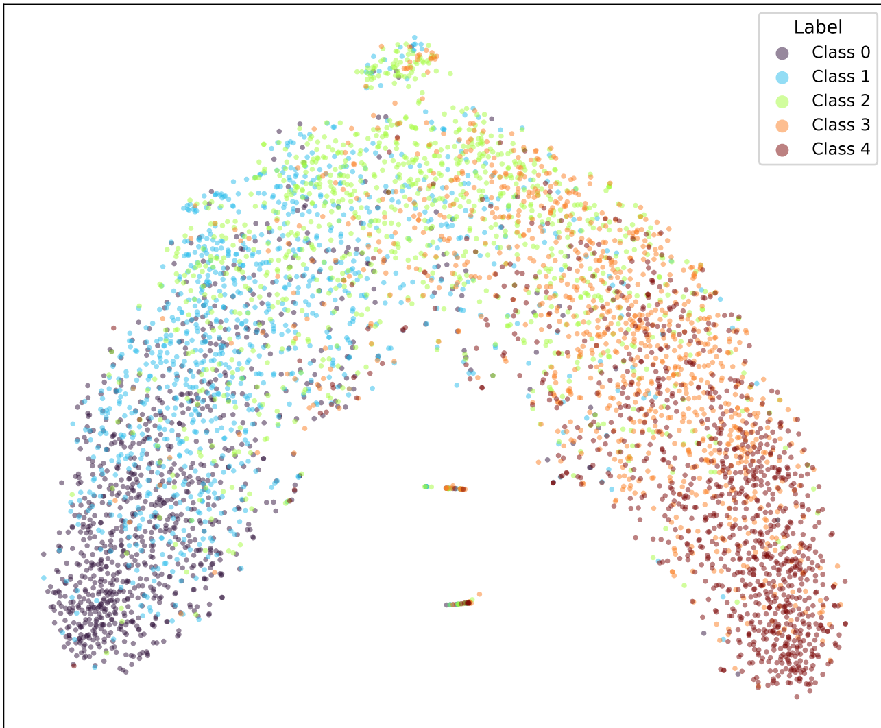
t-SNE | bert-tiny-yelp-k1-adaptive-cosine (epoch 5.0)
