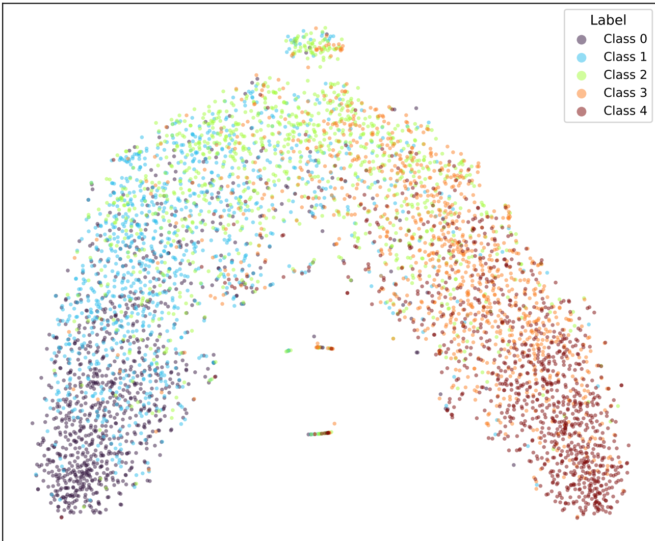
t-SNE | bert-tiny-yelp-k1-adaptive-cosine (epoch 7.0)
