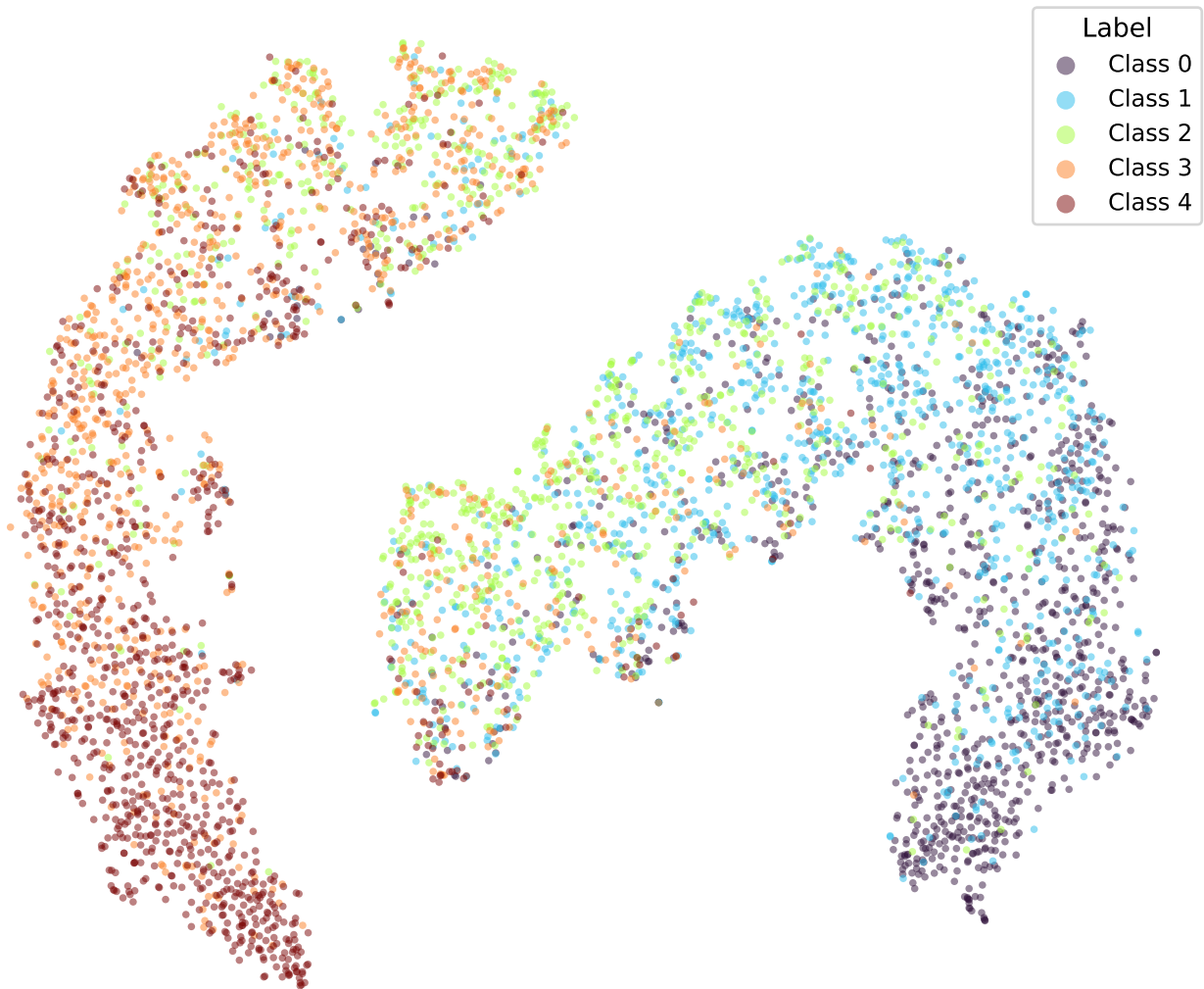
t-SNE | bert-tiny-yelp-k1-adaptive-euclidean (epoch 5.0)
