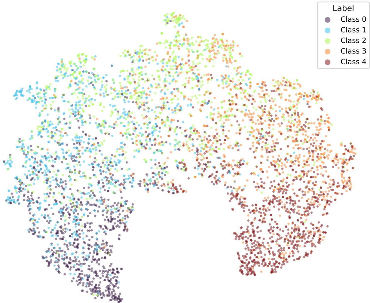
t-SNE | bert-tiny-yelp-k1-fixed-euclidean
