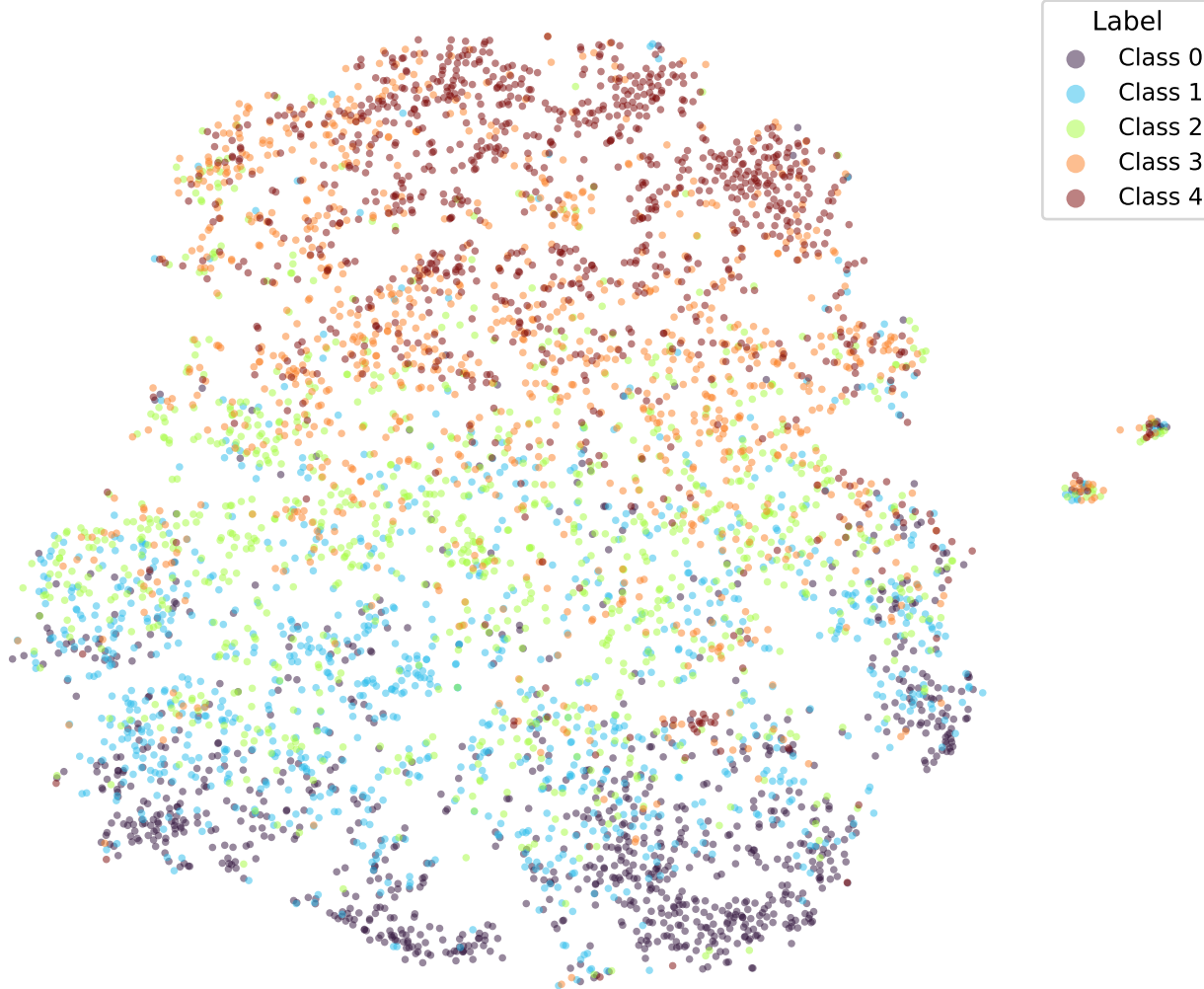
t-SNE | bert-tiny-yelp-k3-fixed-cosine
