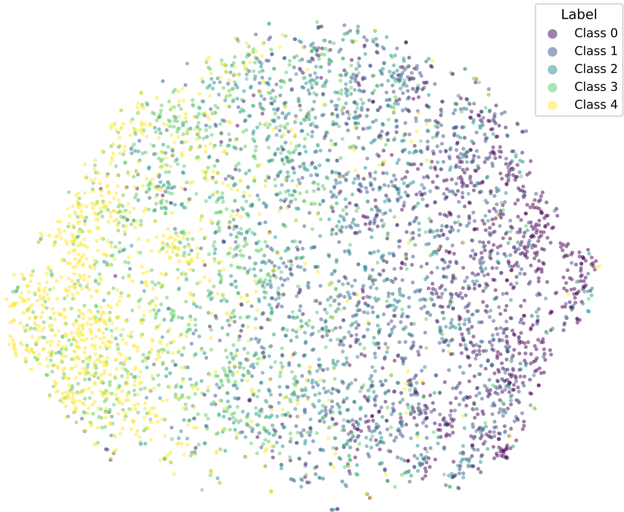
t-SNE | bert-tiny-amazon_reviews-k5-adaptive-cosine
