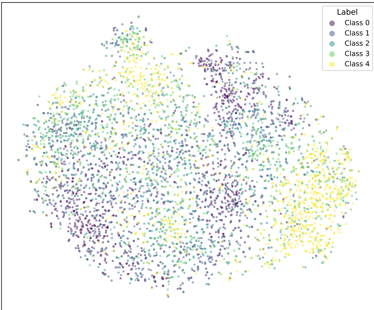
t-SNE | bert-tiny-amazon_reviews-k5-fixed-cosine
