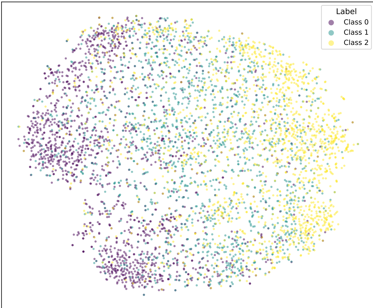
t-SNE | bert-tiny-snli-k3-adaptive-cosine
