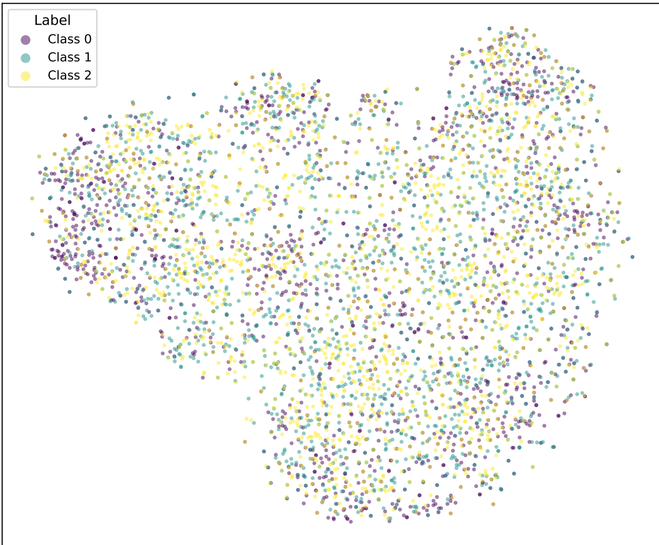
t-SNE | bert-tiny-snli-k3-fixed-euclidean
