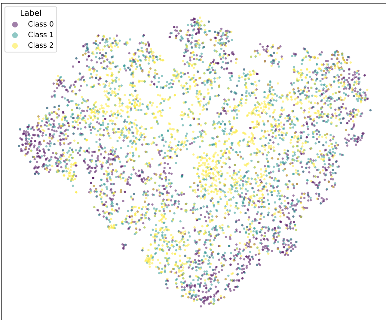
t-SNE | bert-tiny-snli-k5-adaptive-euclidean
