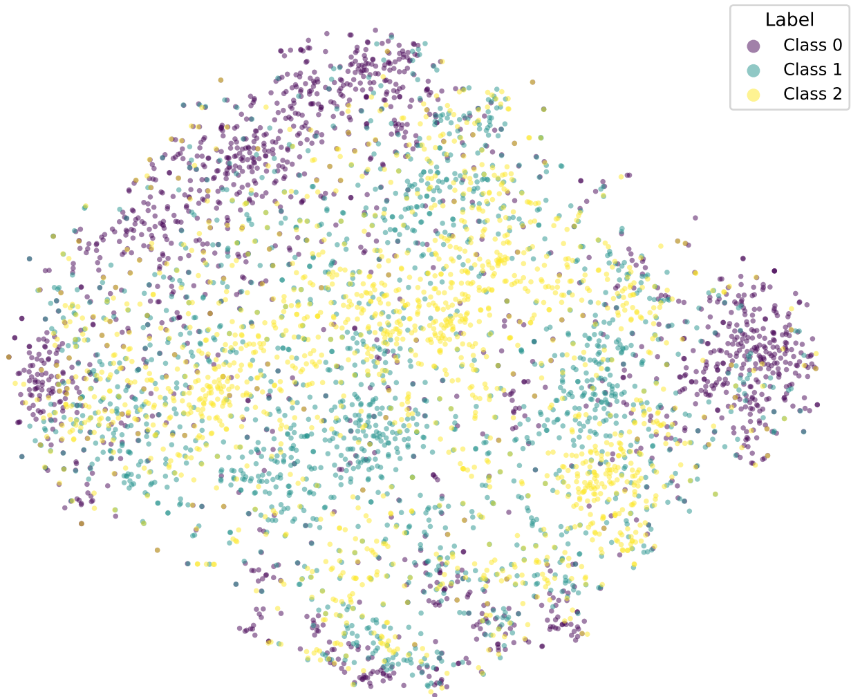
t-SNE | bert-tiny-snli-k5-fixed-cosine
