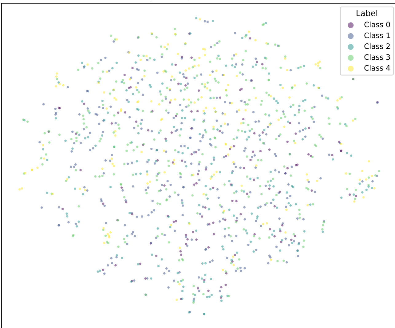
t-SNE | bert-tiny-sst5-k1-fixed-cosine
