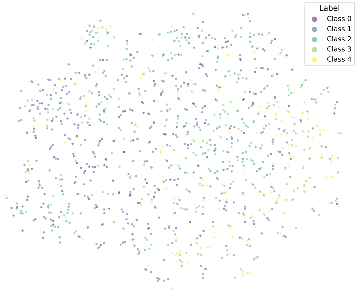
t-SNE | bert-tiny-sst5-k3-adaptive-cosine
