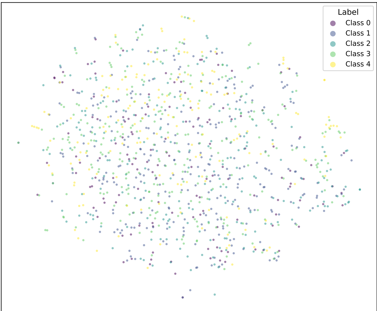
t-SNE | bert-tiny-sst5-k3-adaptive-euclidean
