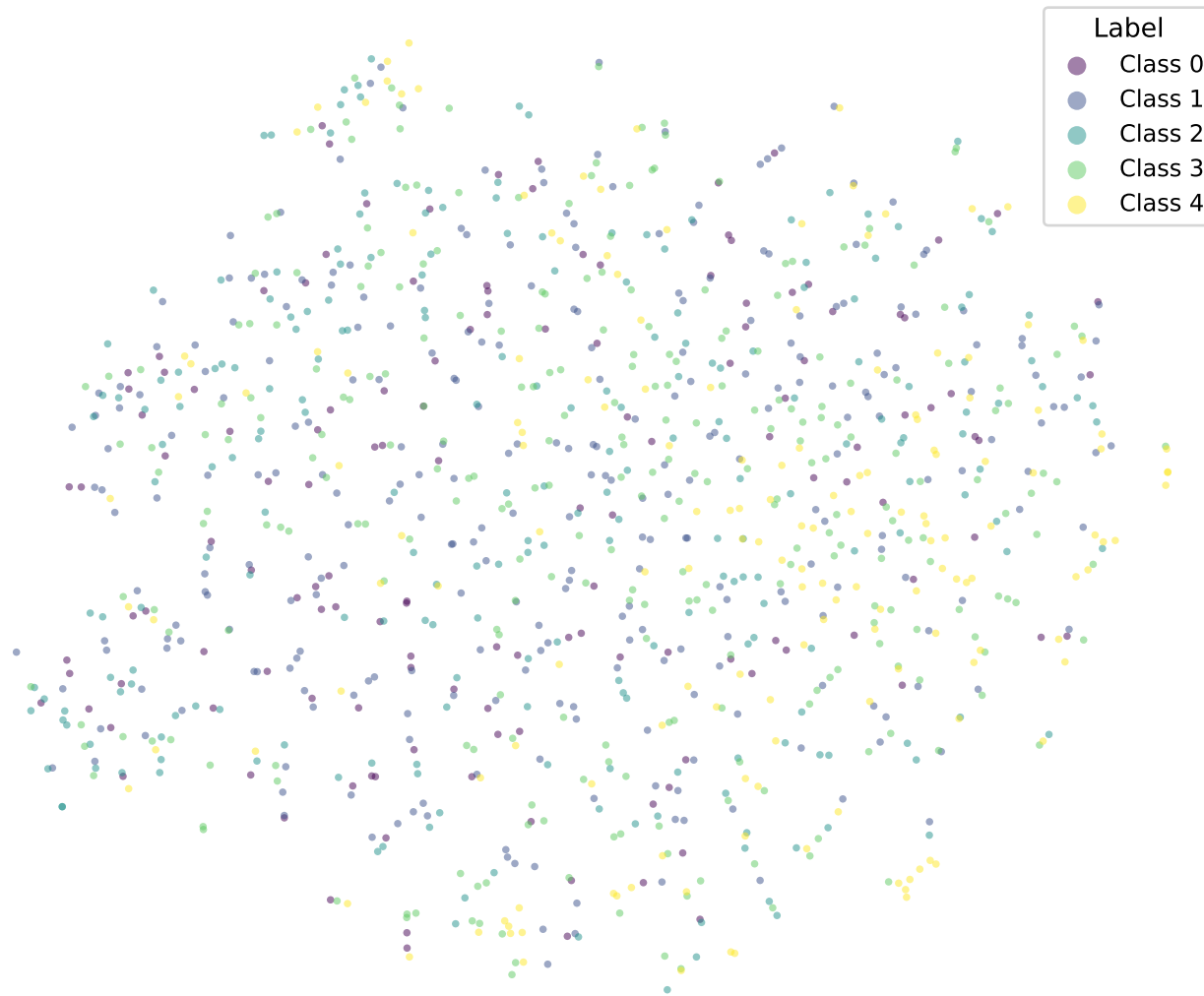
t-SNE | bert-tiny-sst5-k3-fixed-cosine
