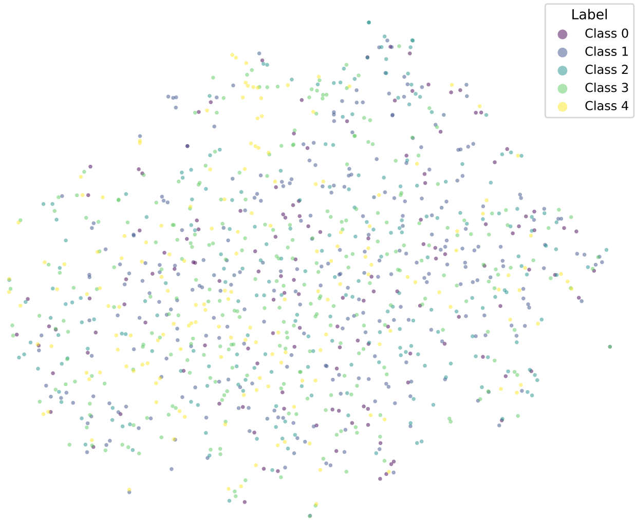
t-SNE | bert-tiny-sst5-k5-adaptive-euclidean
