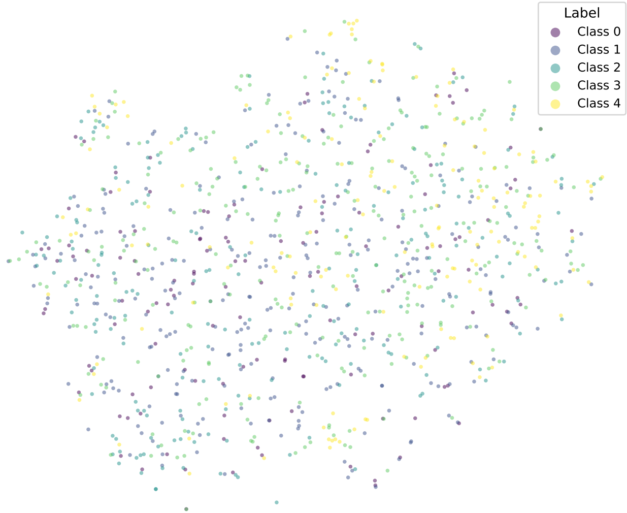
t-SNE | bert-tiny-sst5-k5-fixed-cosine
