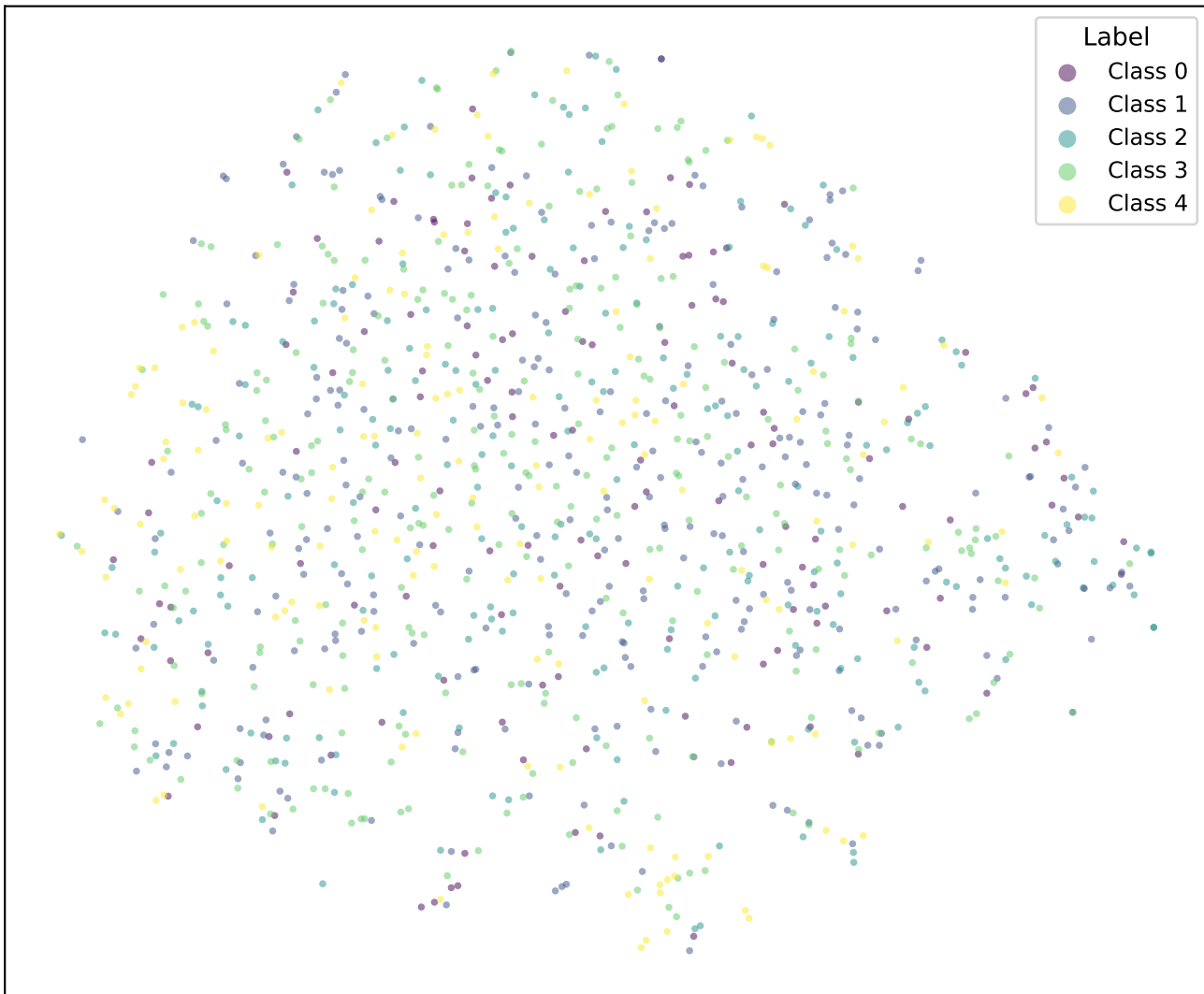
t-SNE | bert-tiny-sst5-k5-fixed-euclidean
