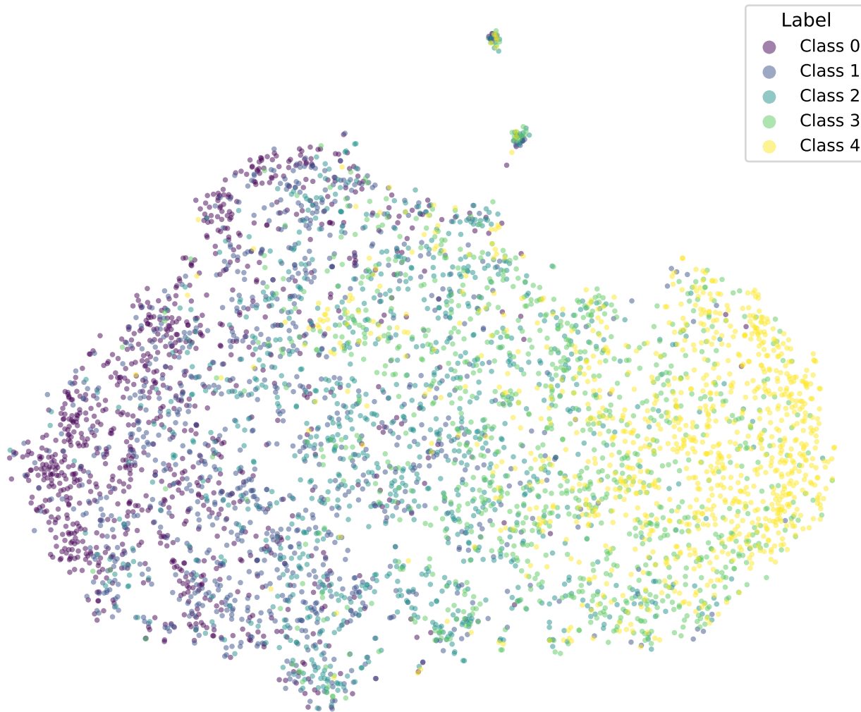
t-SNE | bert-tiny-yelp-k3-adaptive-cosine
