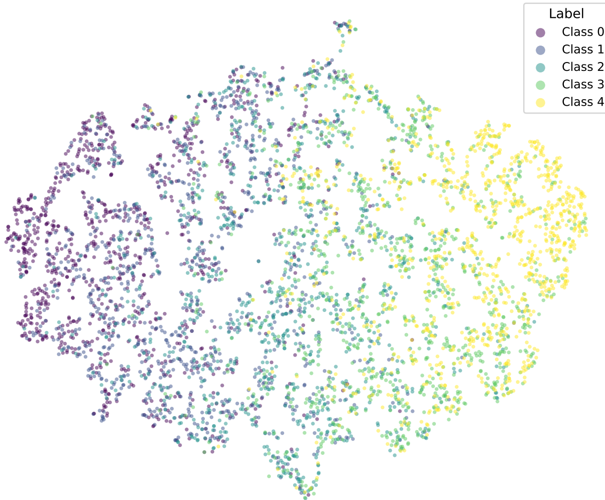
t-SNE | bert-tiny-yelp-k3-adaptive-euclidean
