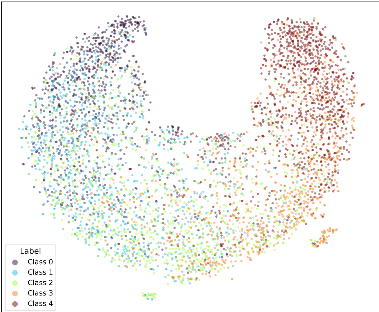
google/bert_uncased_L-2_H-128_A-2-amazon_reviews-BCE-TRIPa1-1 (val)
