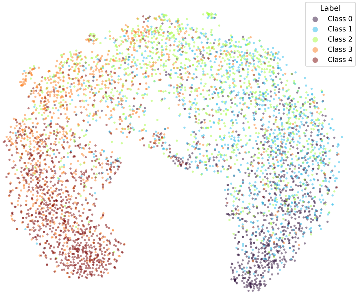
google/bert_uncased_L-2_H-128_A-2-amazon_reviews-BCE-TRIPa1-3 (val)
