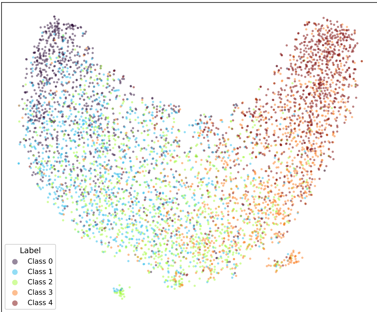
google/bert_uncased_L-2_H-128_A-2-amazon_reviews-CE-TRIPa1-2 (val)
