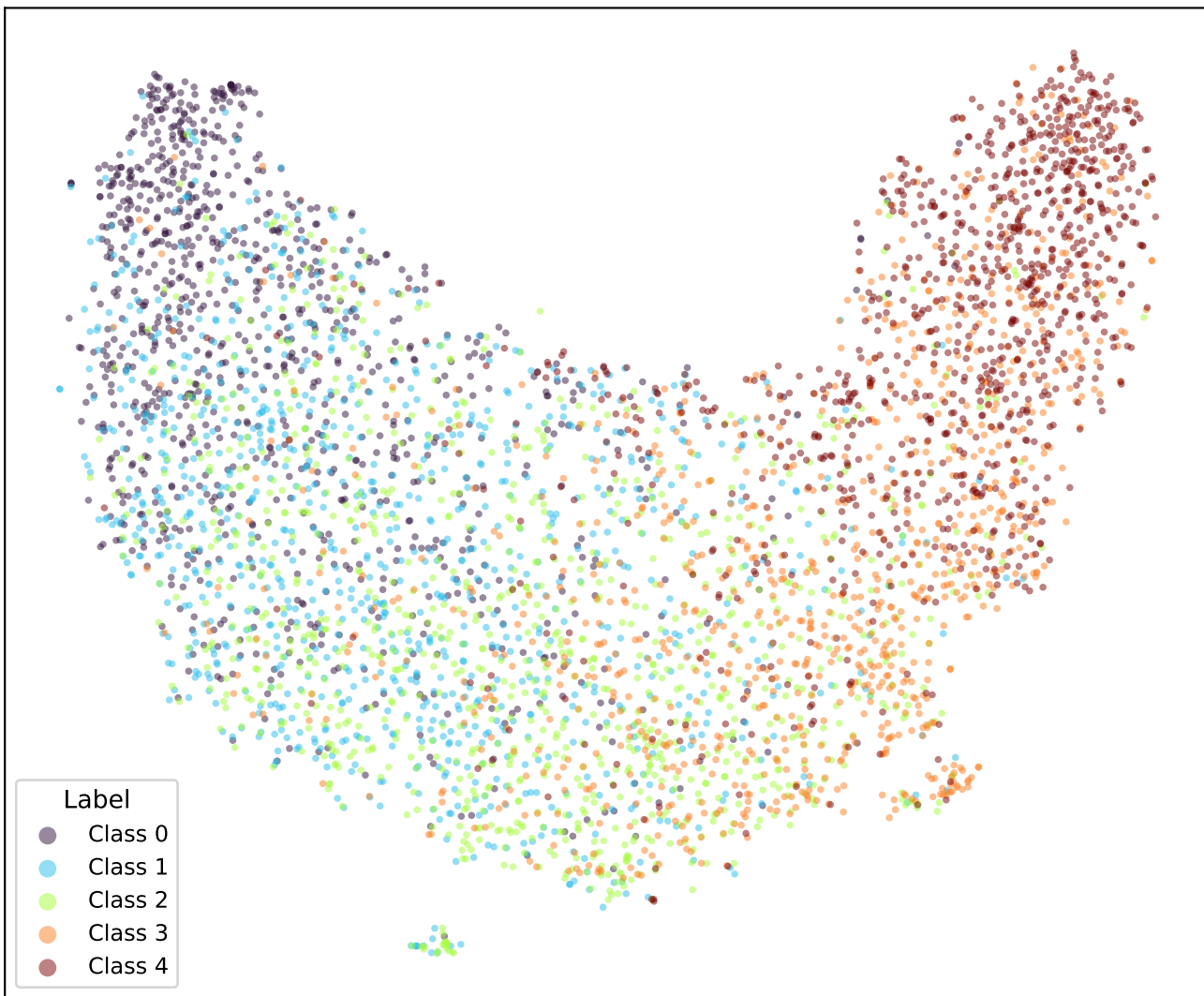
google/bert_uncased_L-2_H-128_A-2-amazon_reviews-CE-TRIPa1-3 (val)
