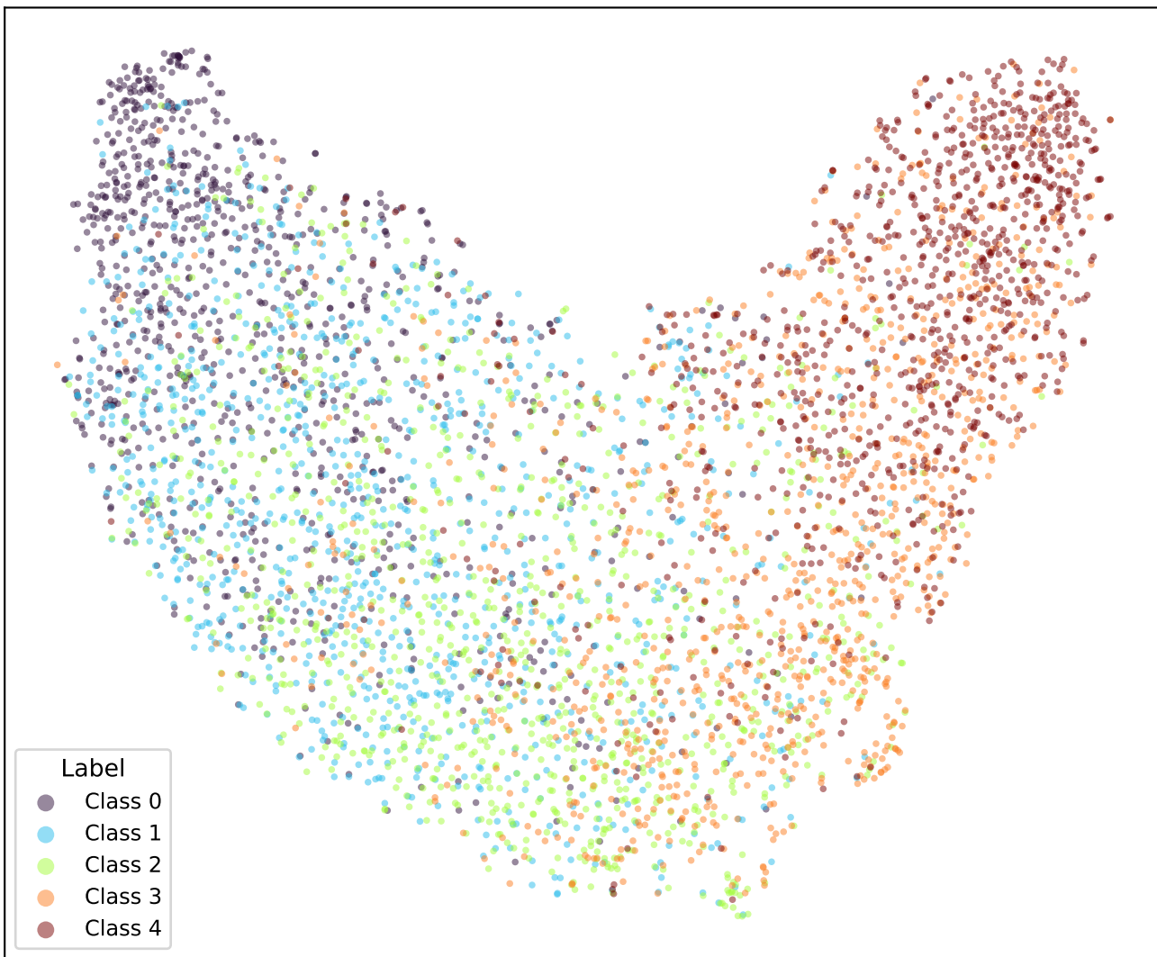
google/bert_uncased_L-2_H-128_A-2-amazon_reviews-CE-TRIPa1-4 (val)
