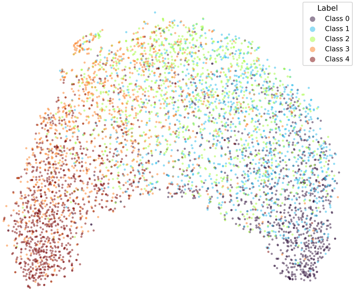
google/bert_uncased_L-2_H-128_A-2-amazon_reviews-CE-TRIPa1-5 (val)
