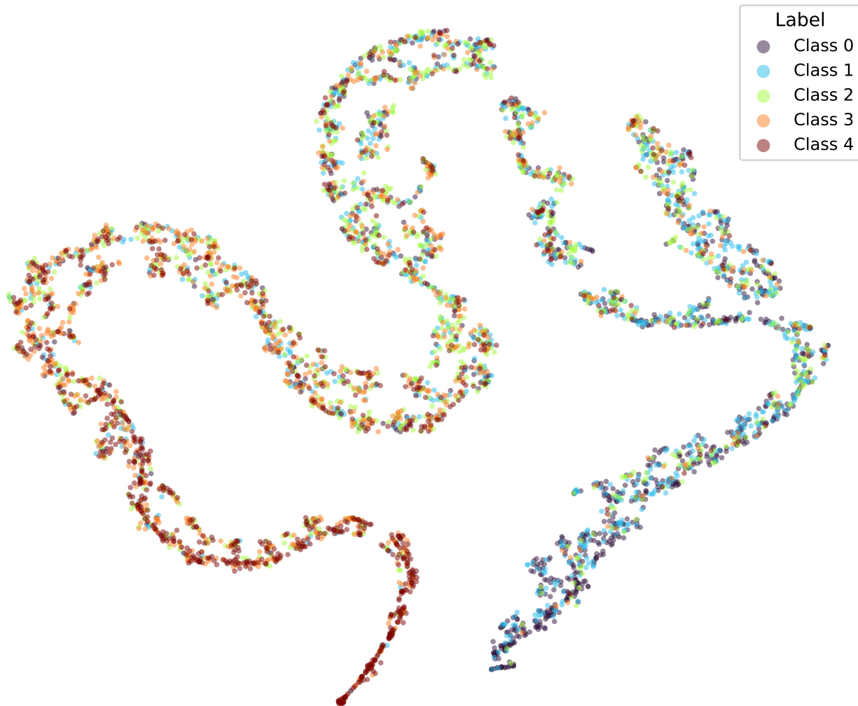
google/bert_uncased_L-2_H-128_A-2-amazon_reviews-CORAL-TRIPa1-1 (val)
