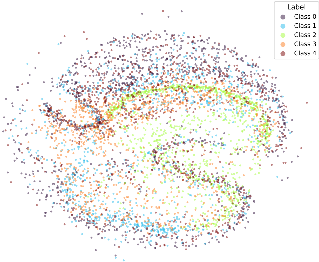
google/bert_uncased_L-2_H-128_A-2-amazon_reviews-CORAL-TRIPa1-3 (val)
