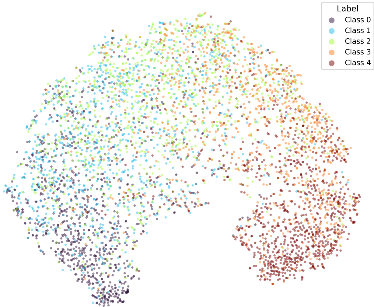
google/bert_uncased_L-2_H-128_A-2-amazon_reviews-CORN-1 (val)
